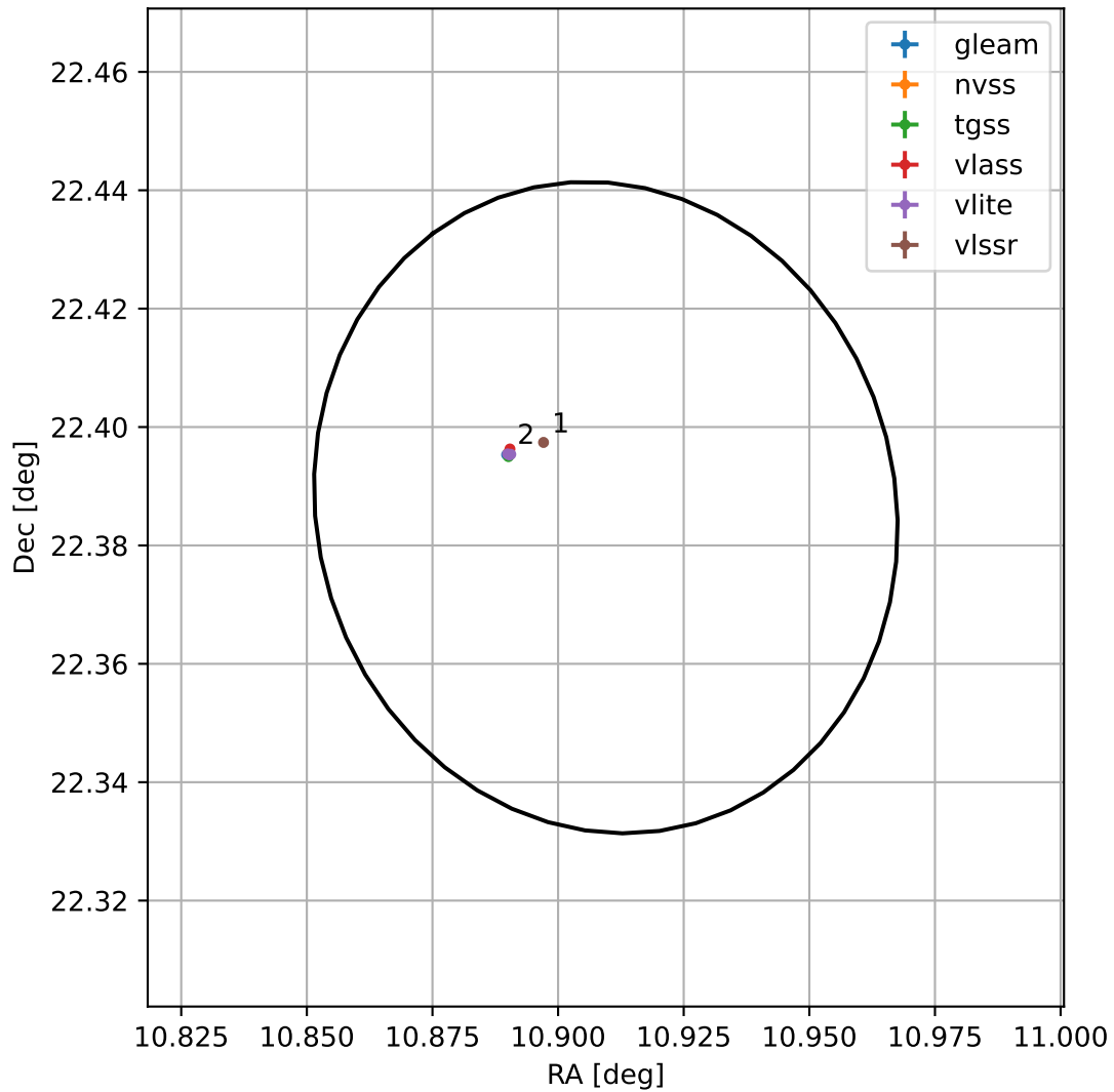
4FGL J0043.6+2223
