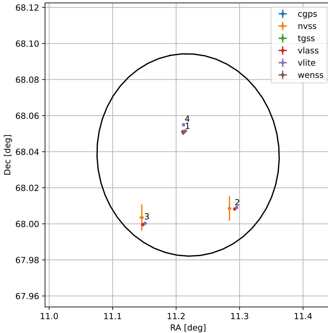
4FGL J0044.8+6802
