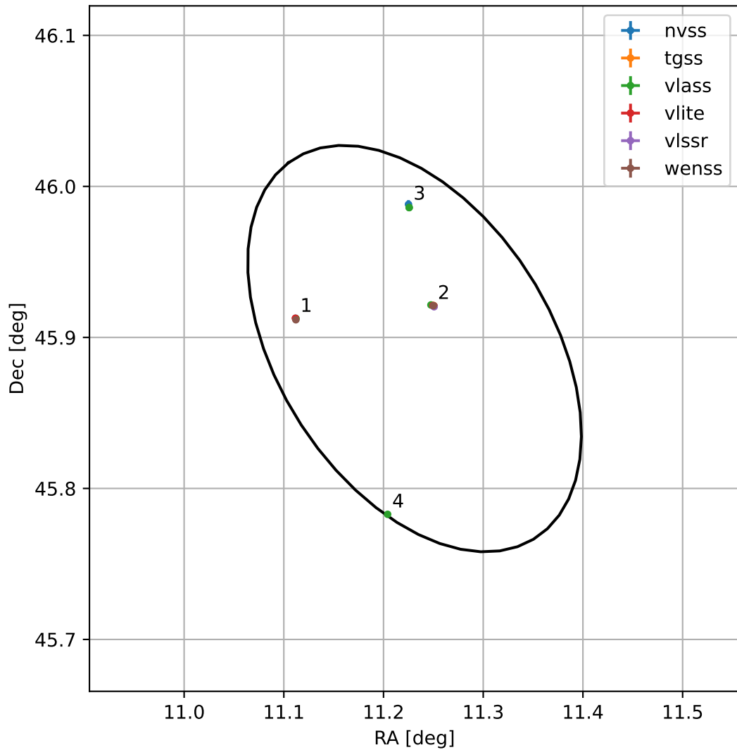
4FGL J0044.9+4553
