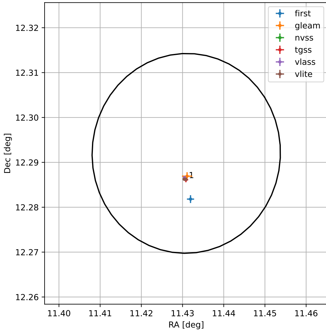
4FGL J0045.7+1217
