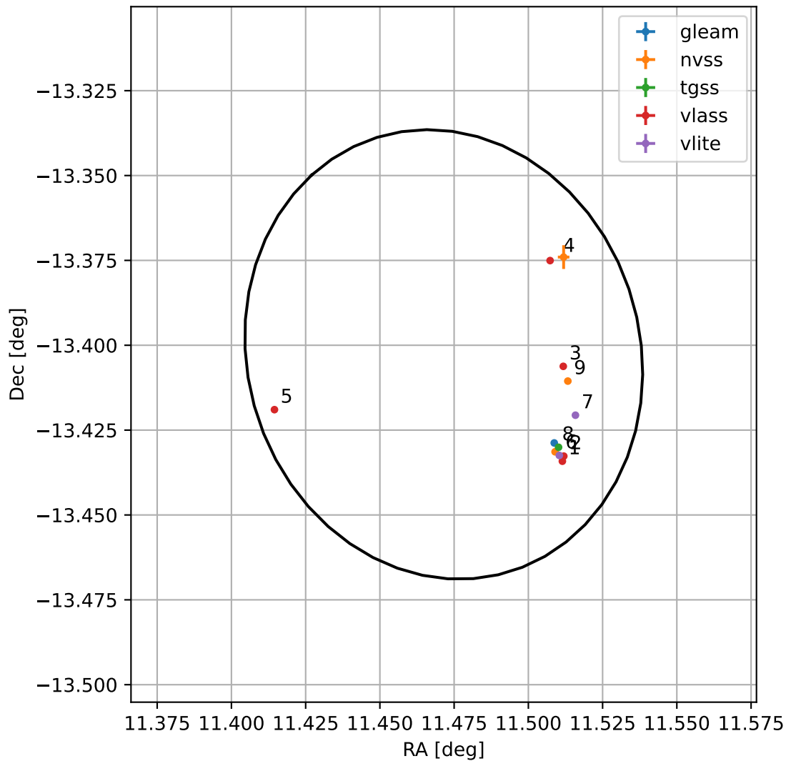
4FGL J0045.8-1324
