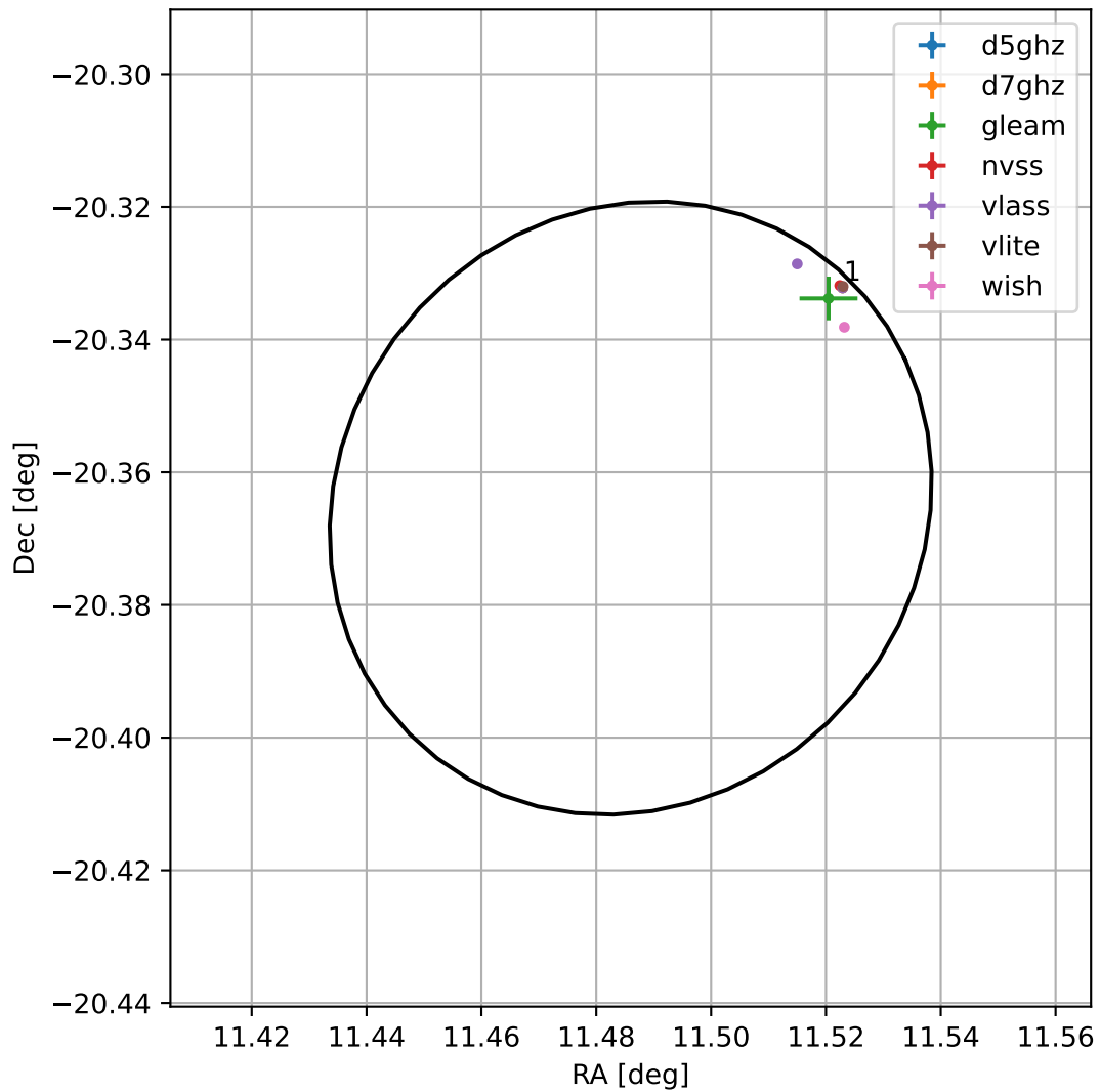
4FGL J0045.9-2021
