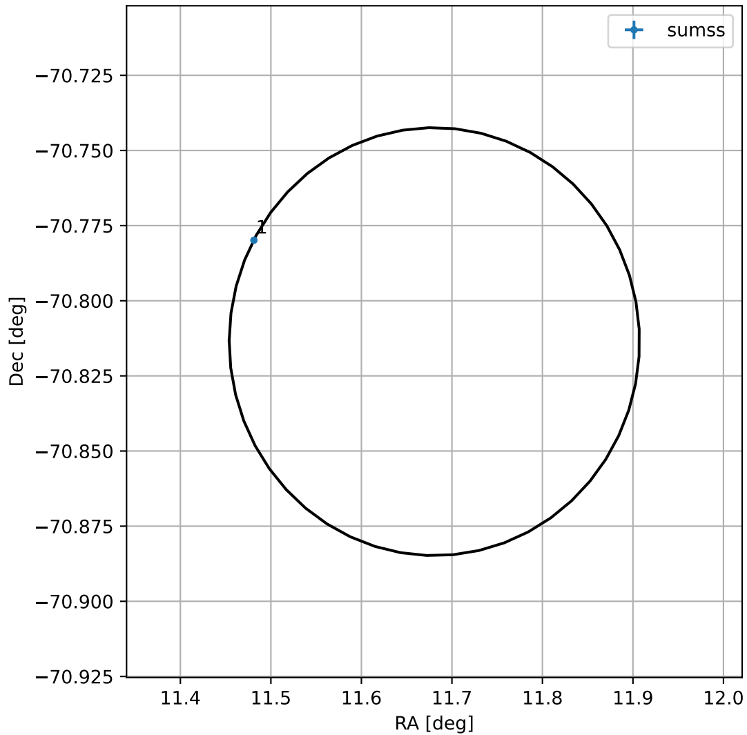
4FGL J0046.7-7048
