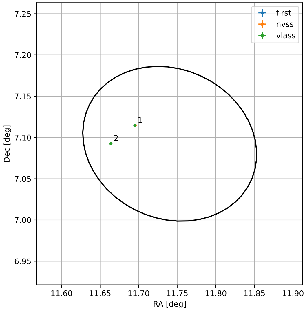
4FGL J0046.9+0705
