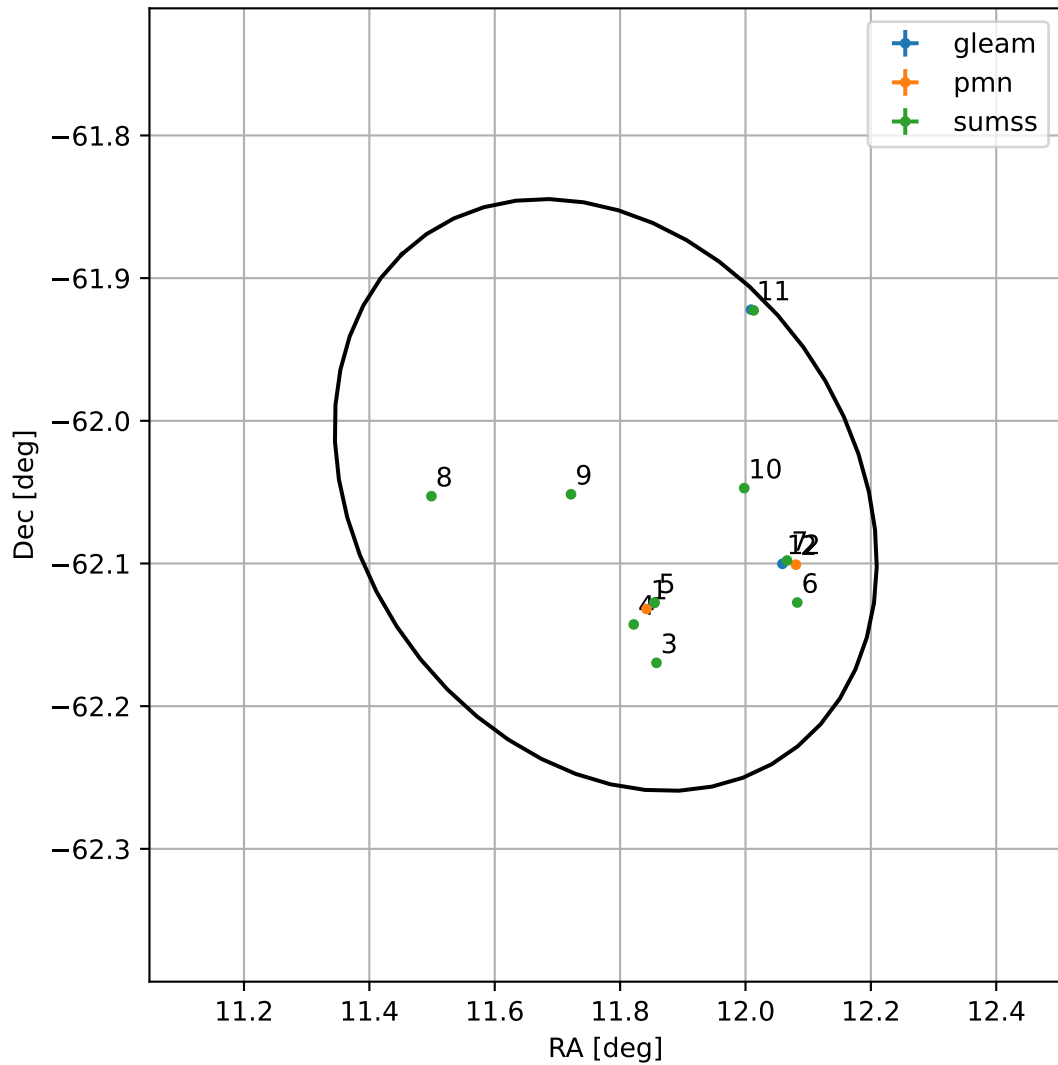
4FGL J0047.1-6203
