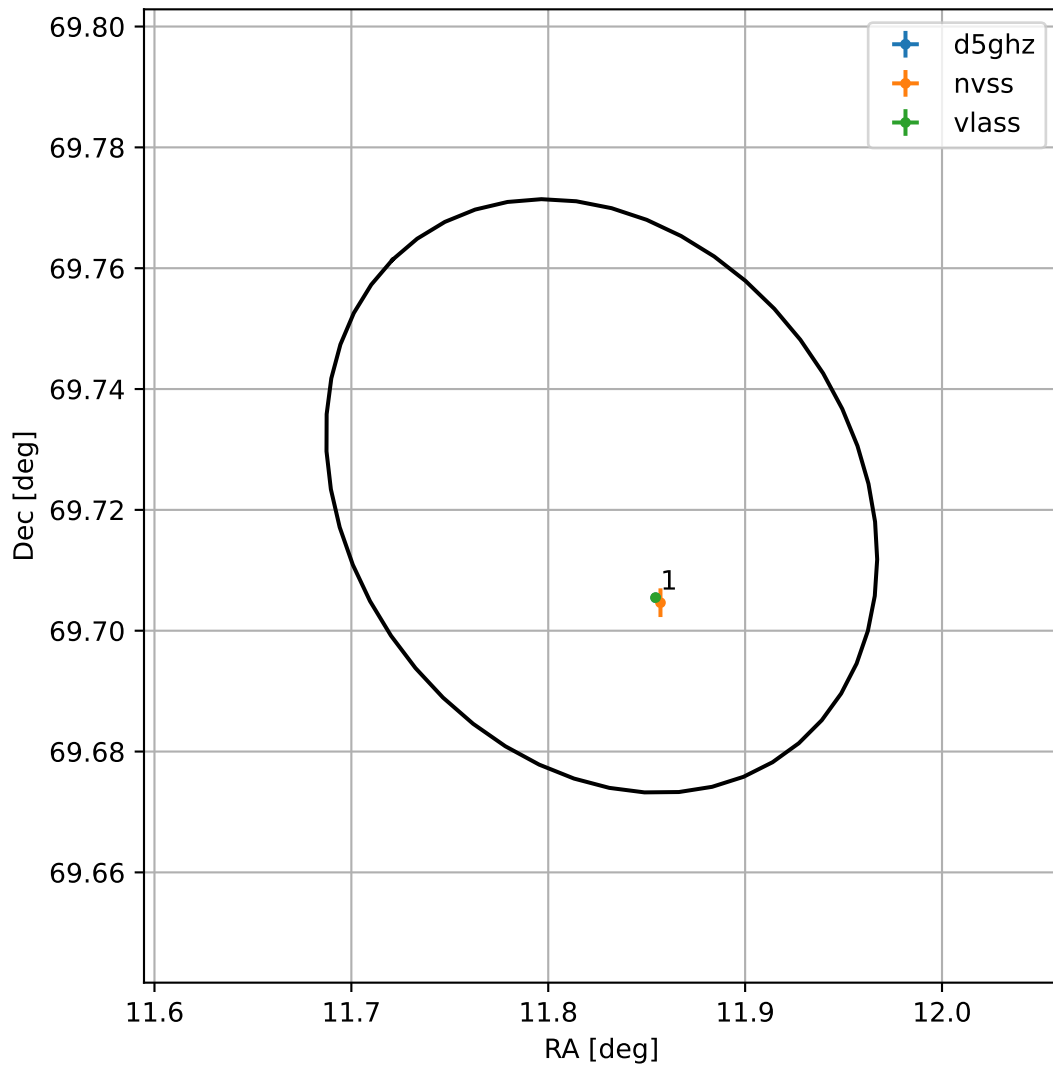
4FGL J0047.3+6943
