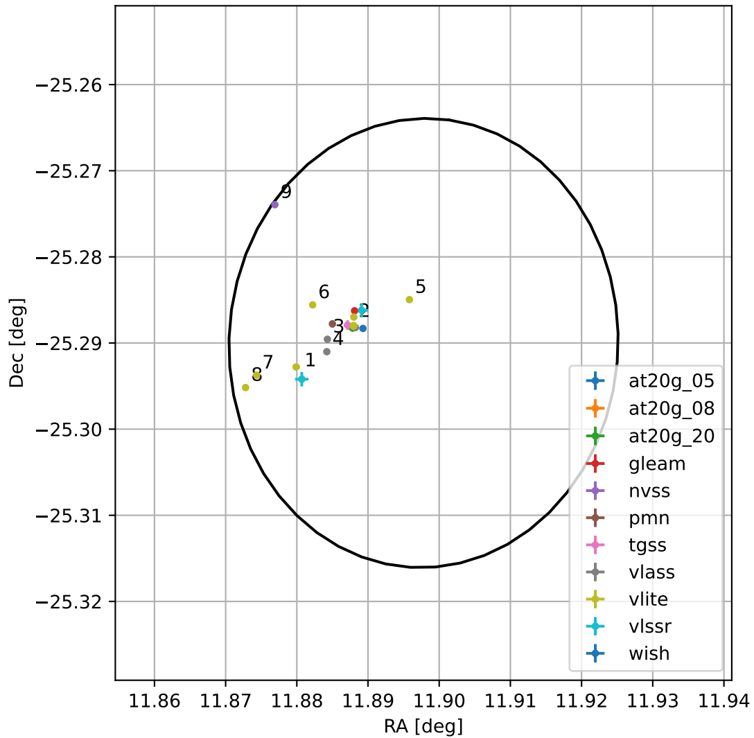
4FGL J0047.5-2517
