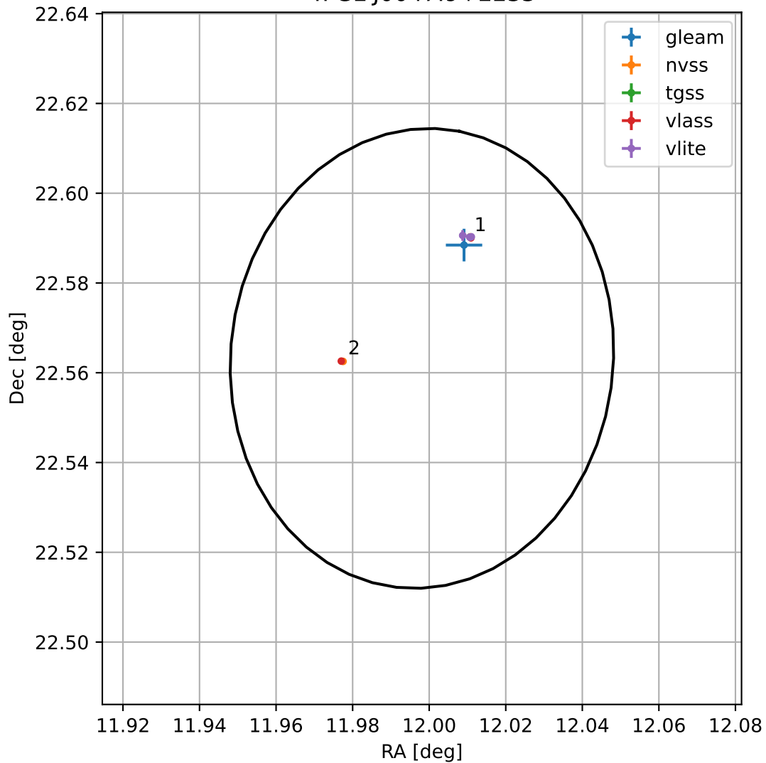
4FGL J0047.9+2233
