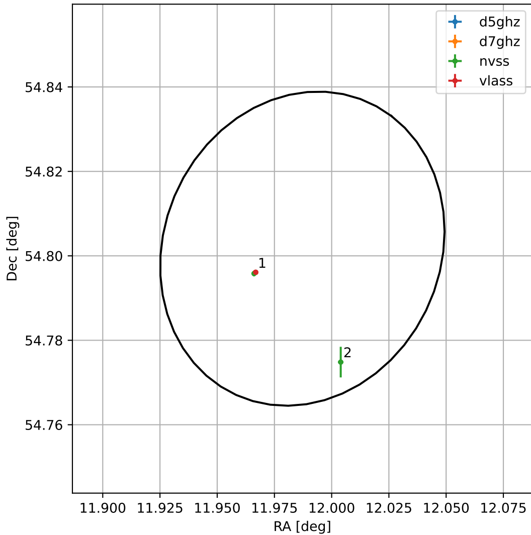
4FGL J0047.9+5448
