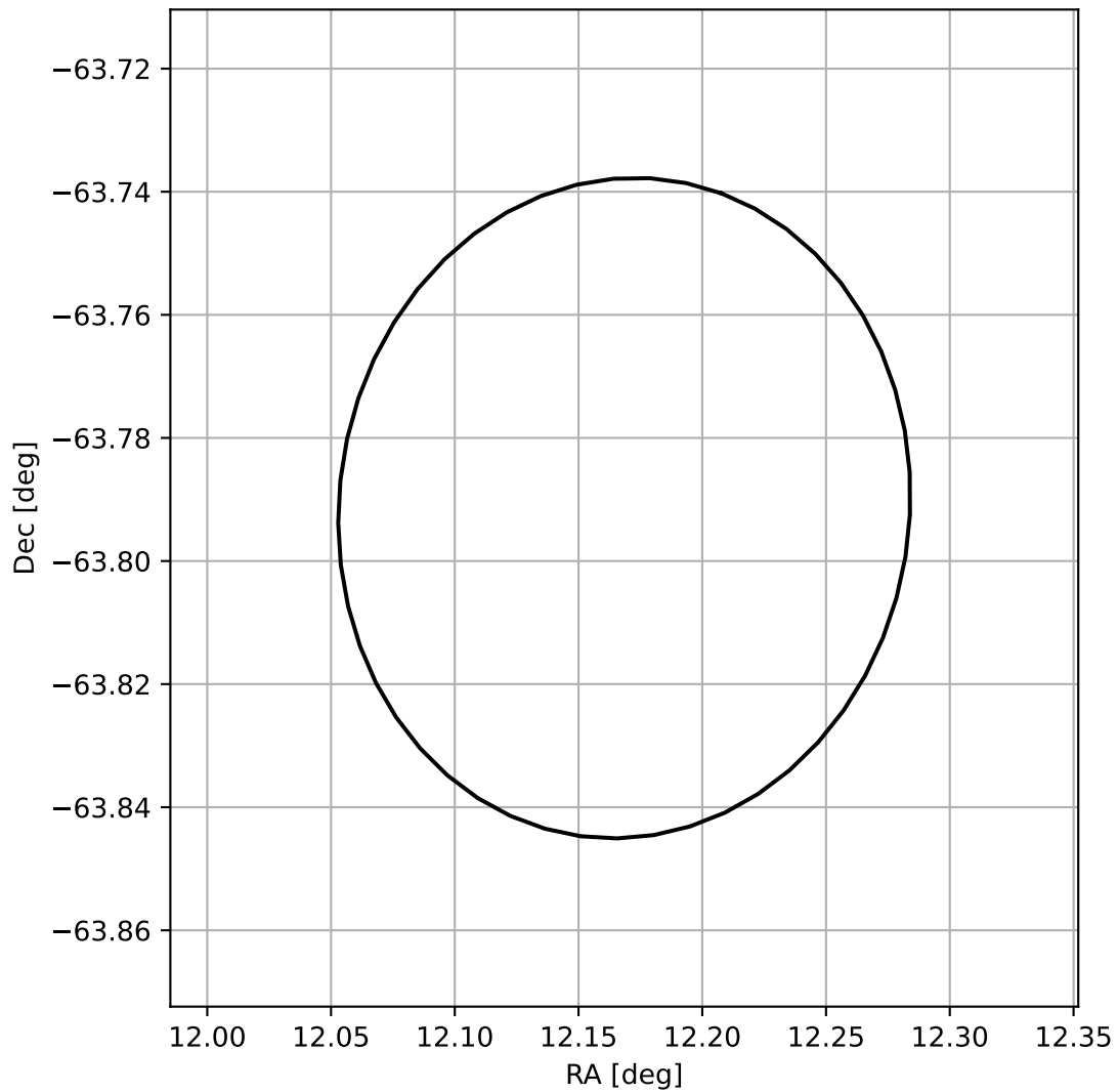
4FGL J0048.6-6347
