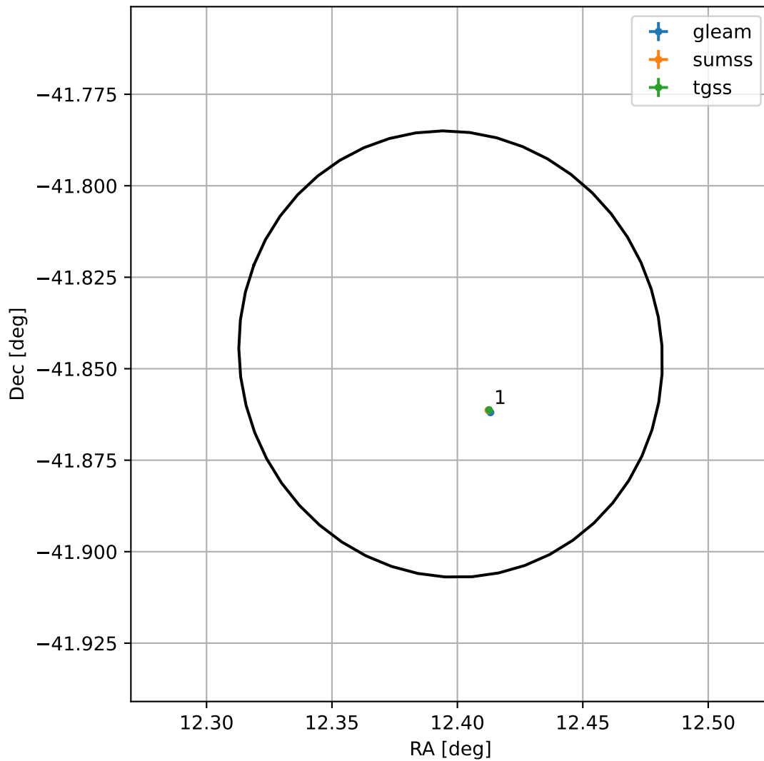
4FGL J0049.5-4150
