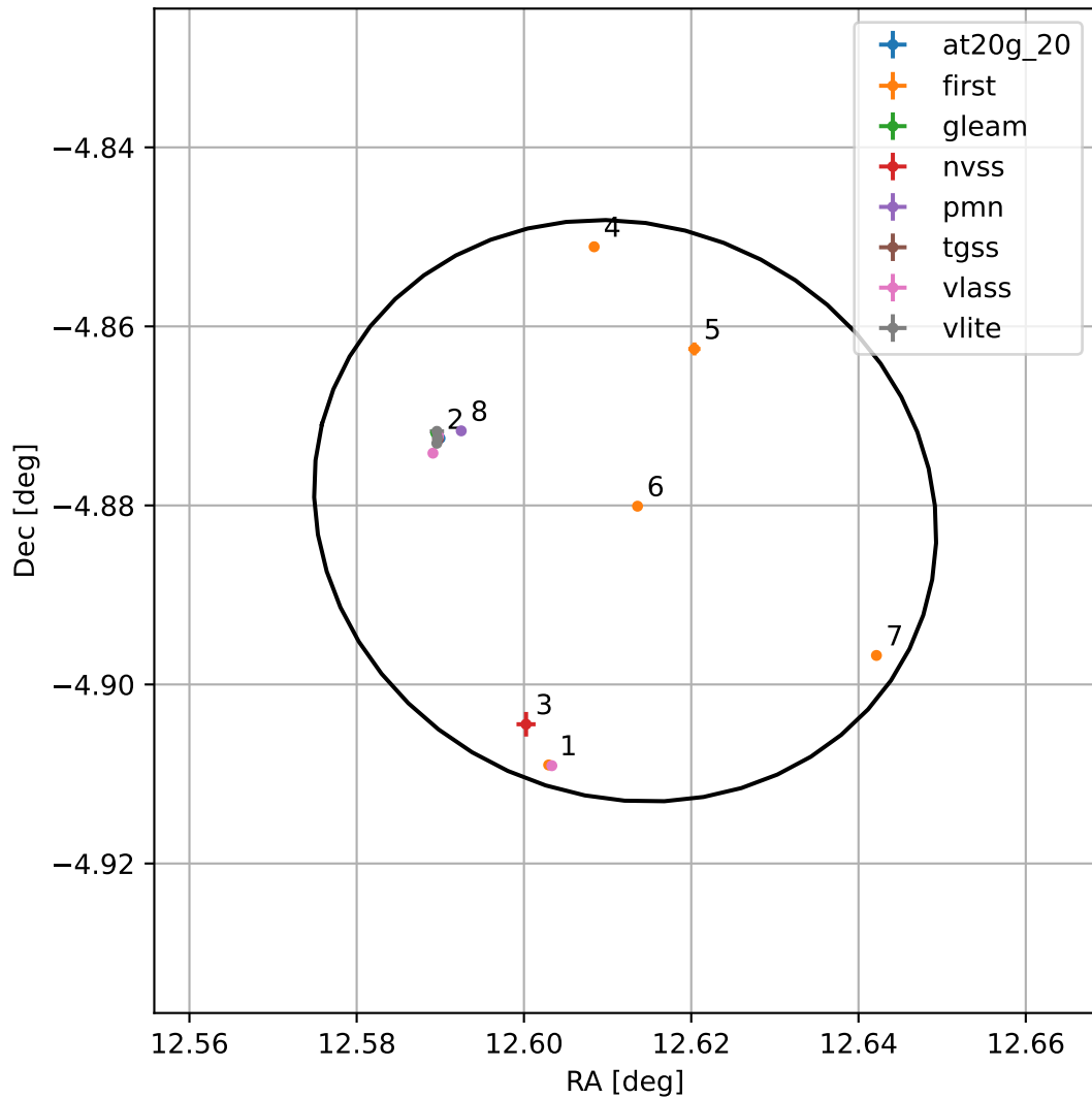
4FGL J0050.4-0452
