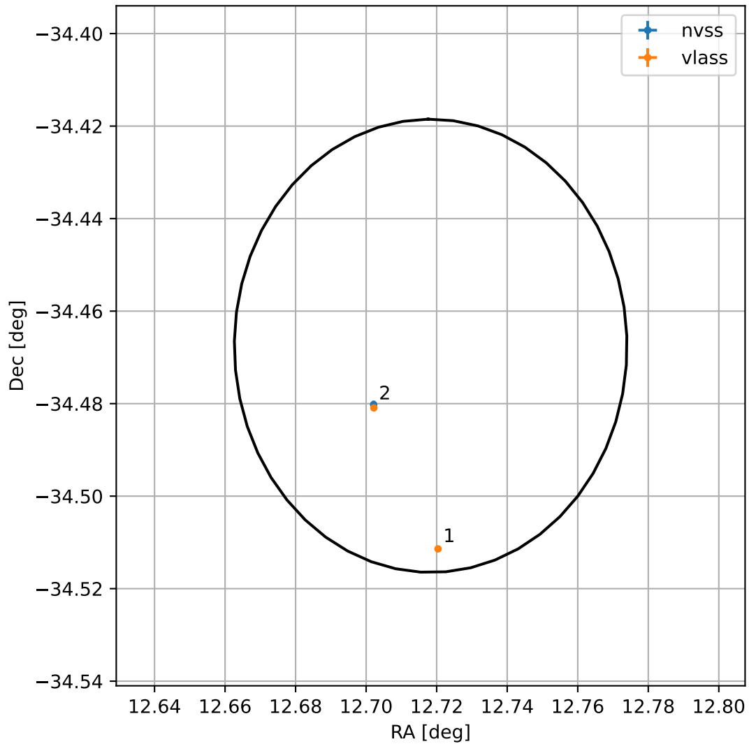
4FGL J0050.8-3428
