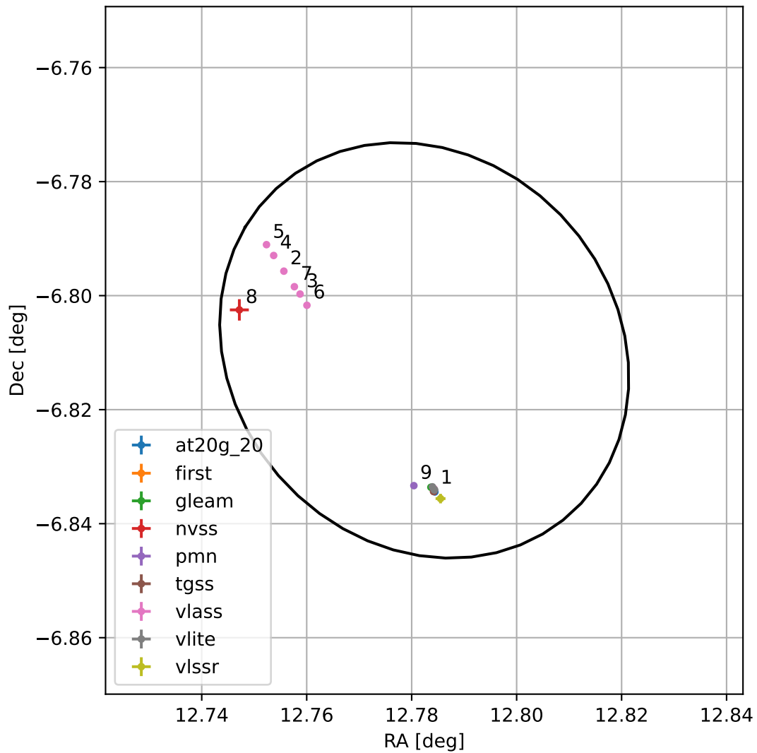
4FGL J0051.1-0648
