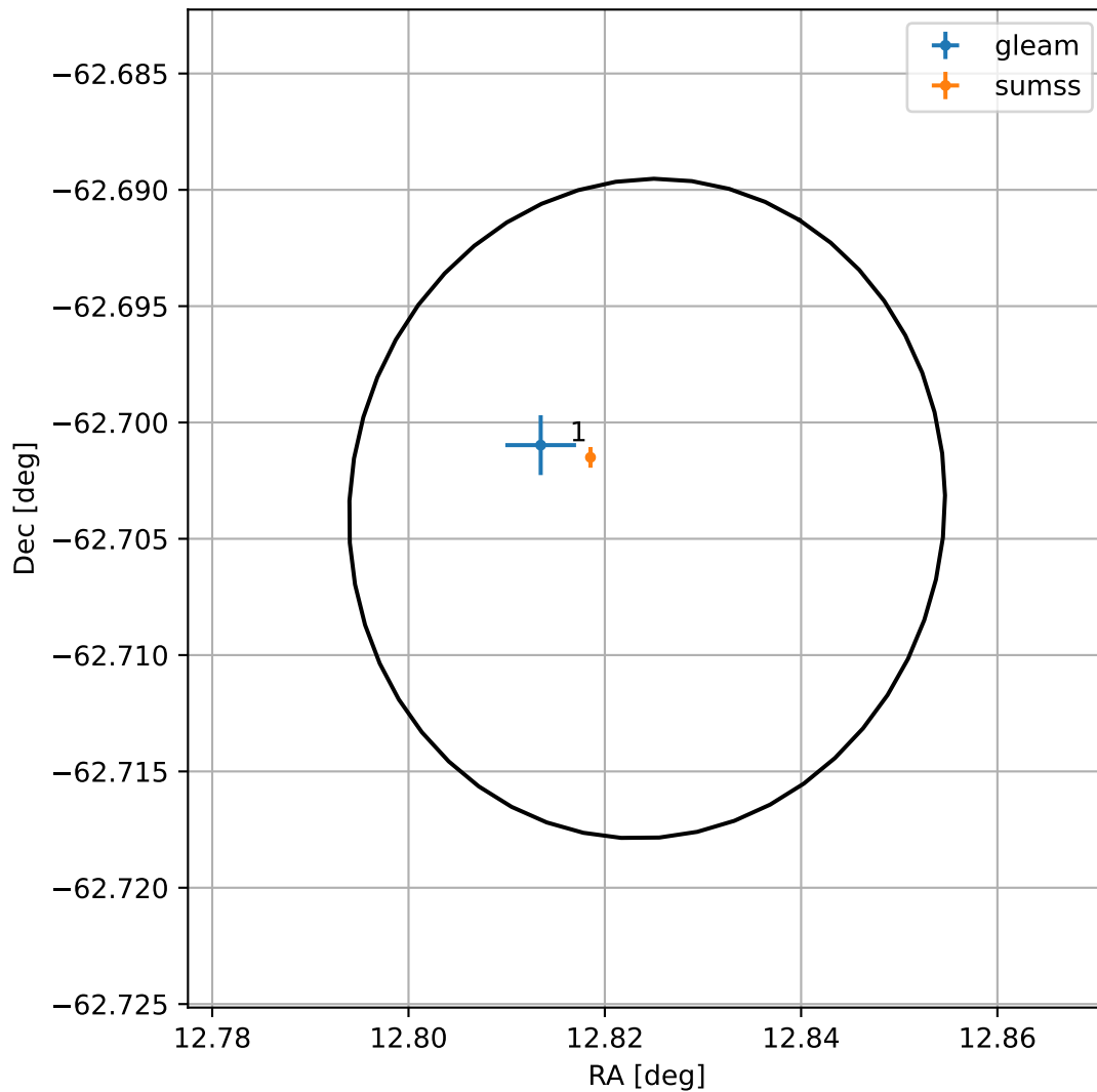
4FGL J0051.2-6242
