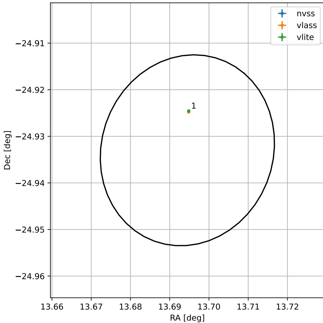
4FGL J0054.7-2455
