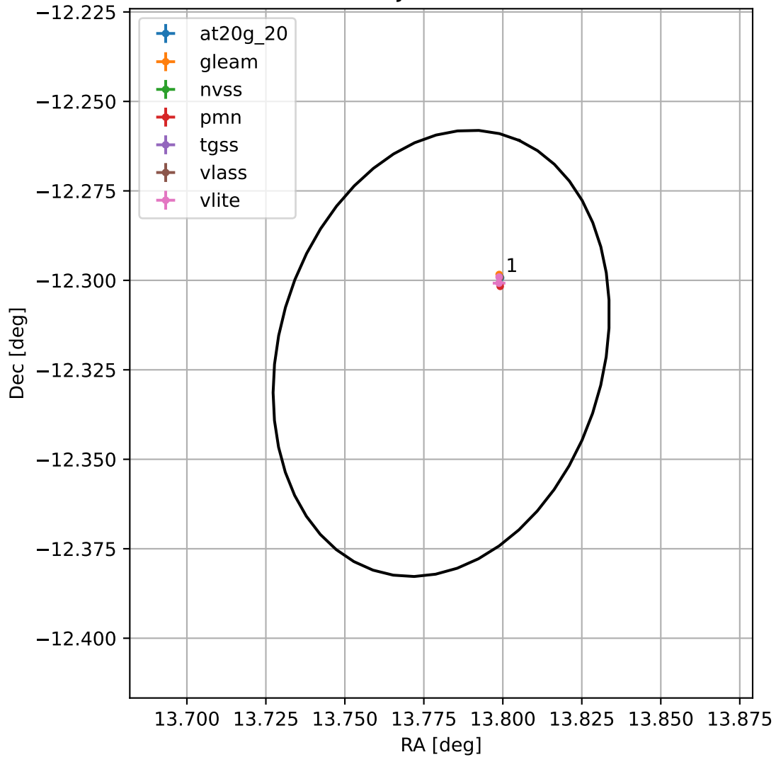
4FGL J0055.1-1219
