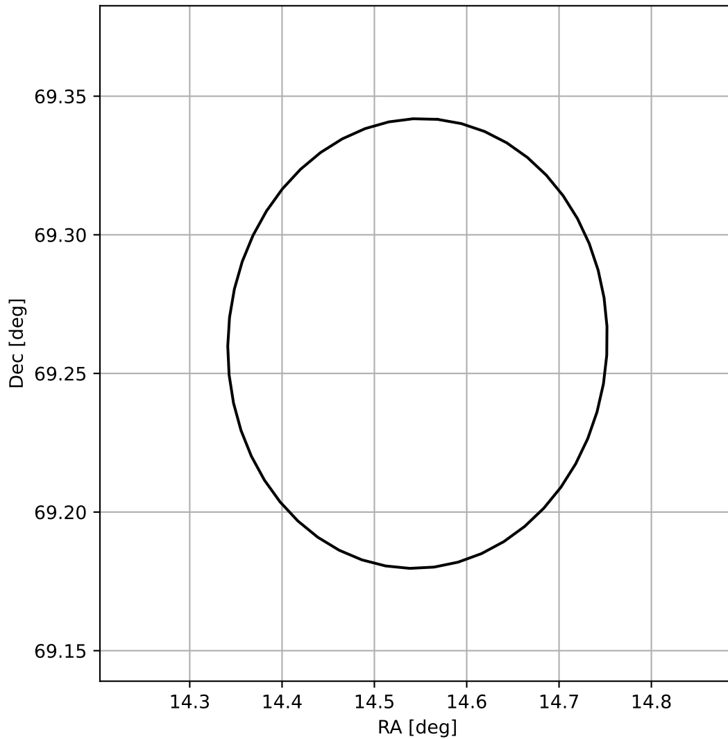
4FGL J0058.1+6915
