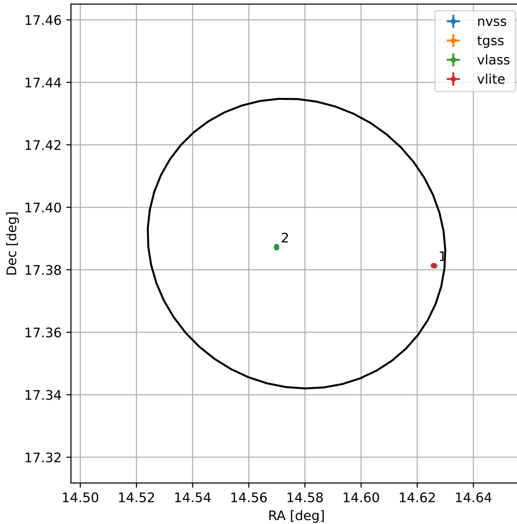
4FGL J0058.3+1723
