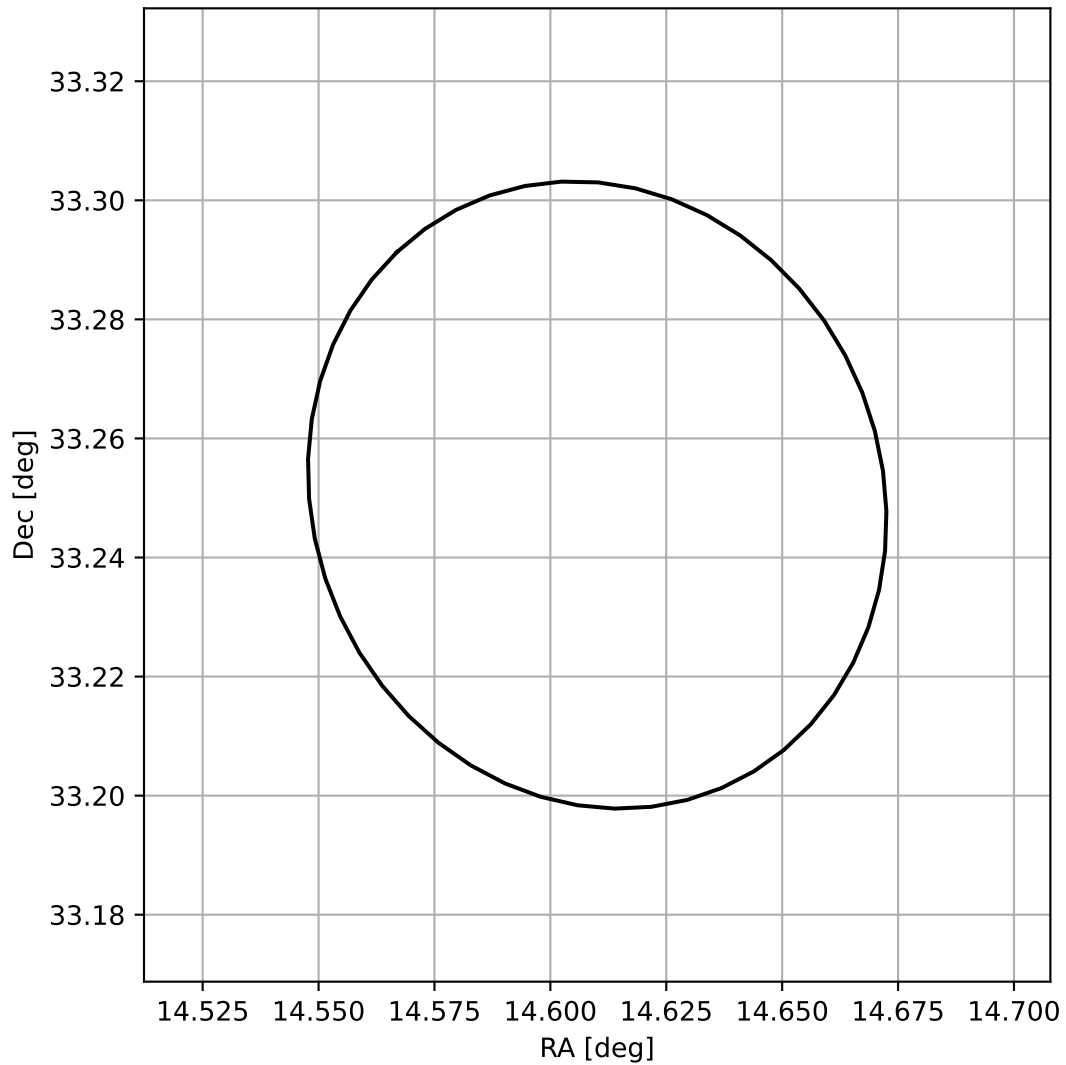
4FGL J0058.4+3315
