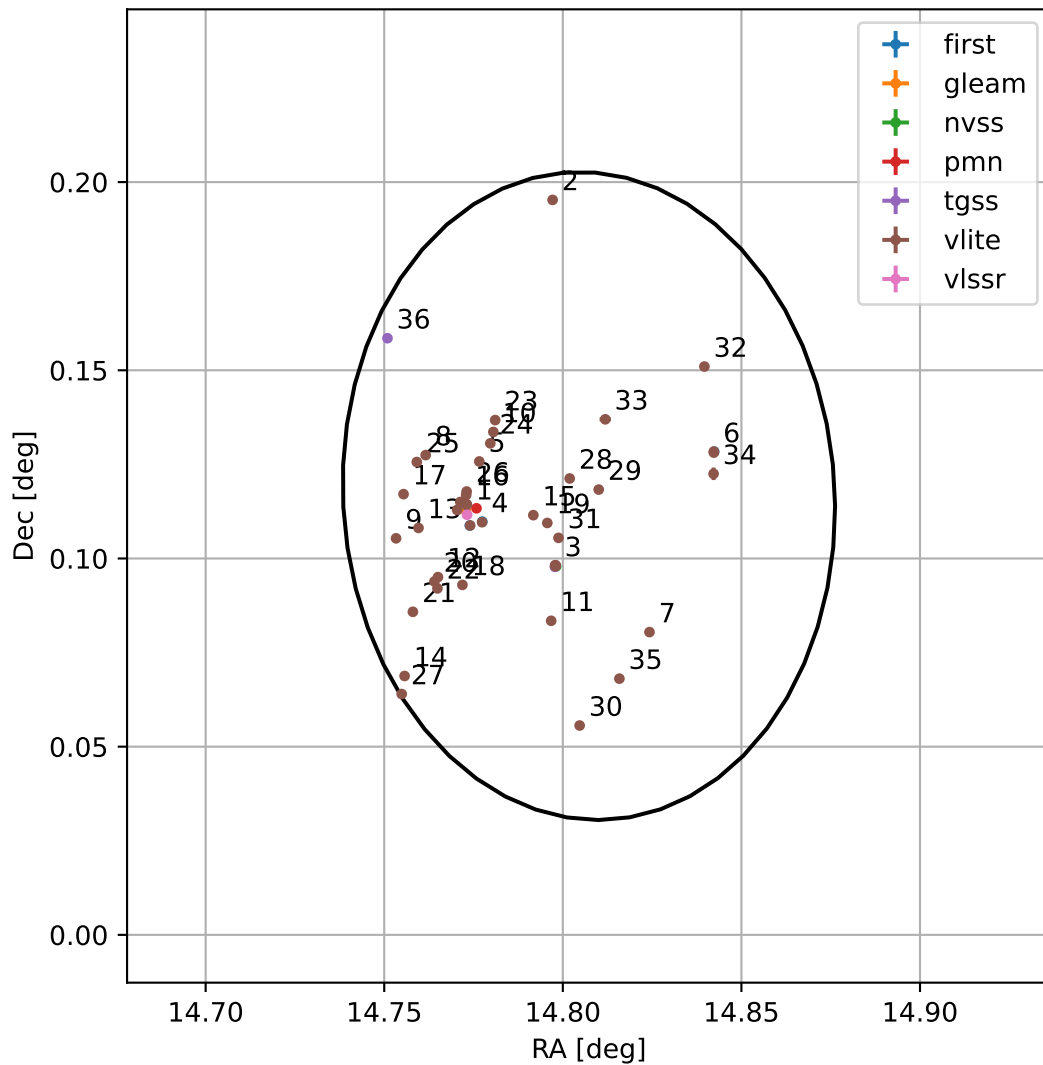
4FGL J0059.2+0006
