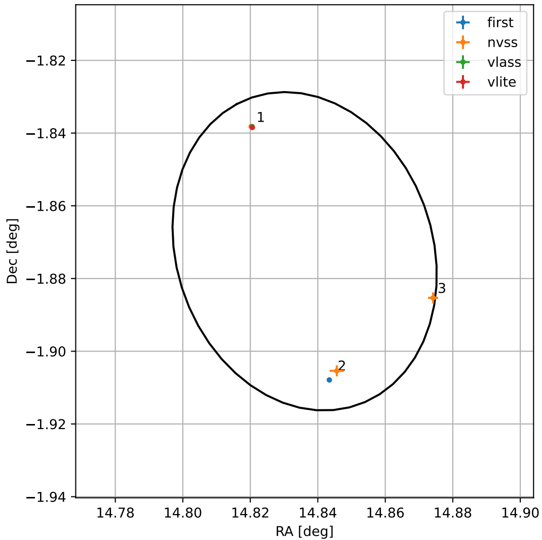
4FGL J0059.3-0152
