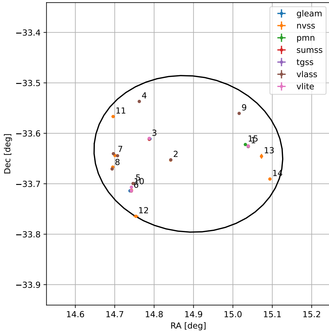
4FGL J0059.5-3338
