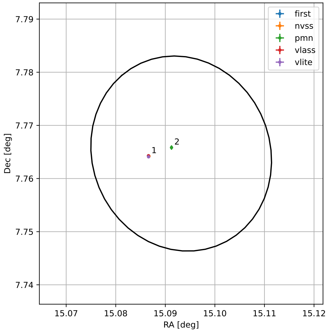
4FGL J0100.3+0745
