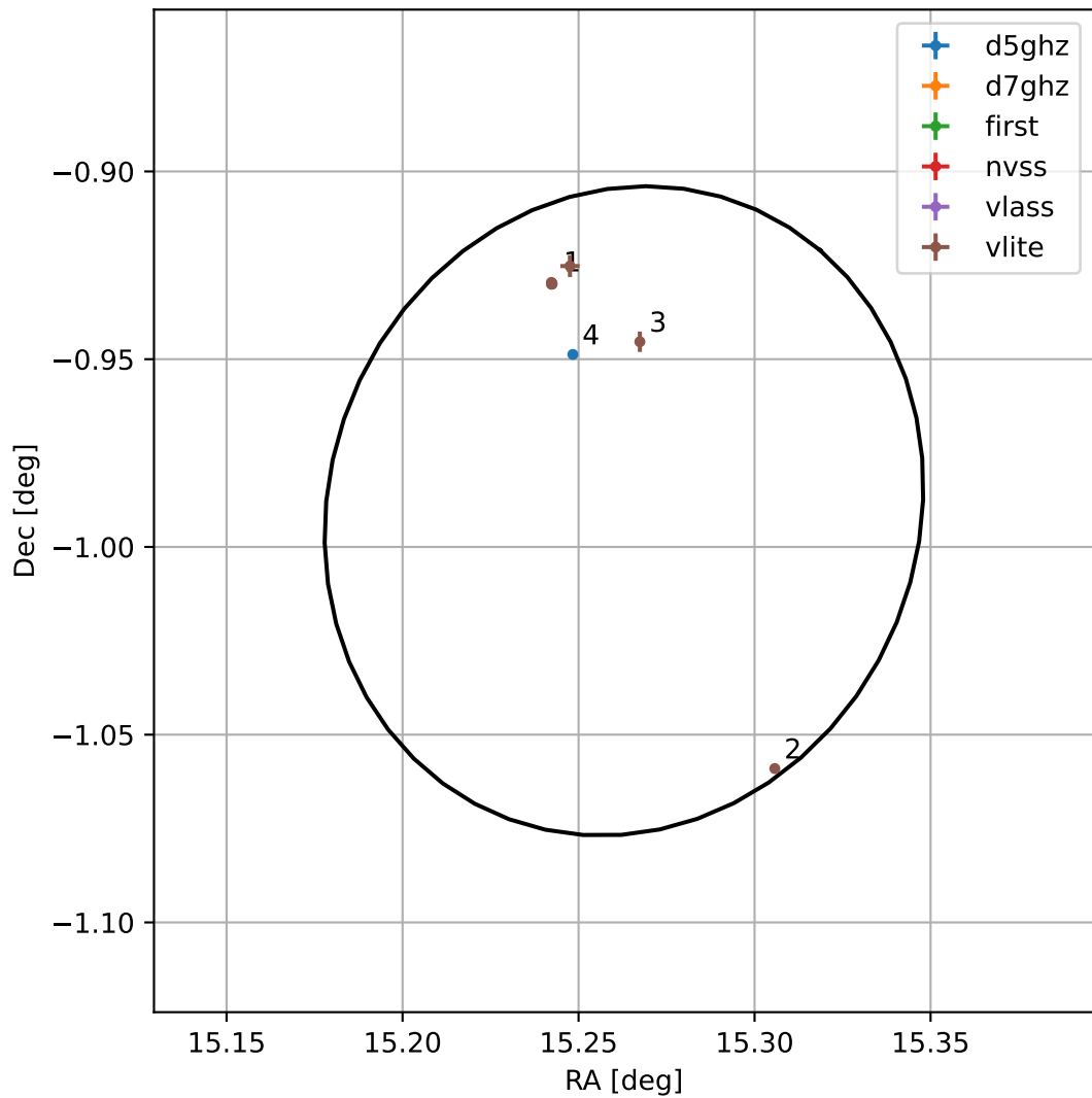
4FGL J0101.0-0059
