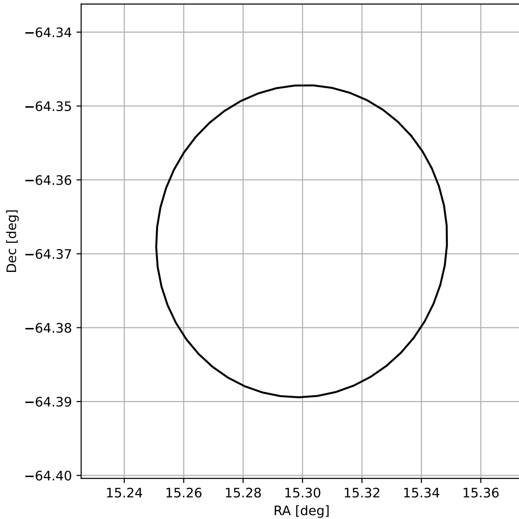
4FGL J0101.1-6422
