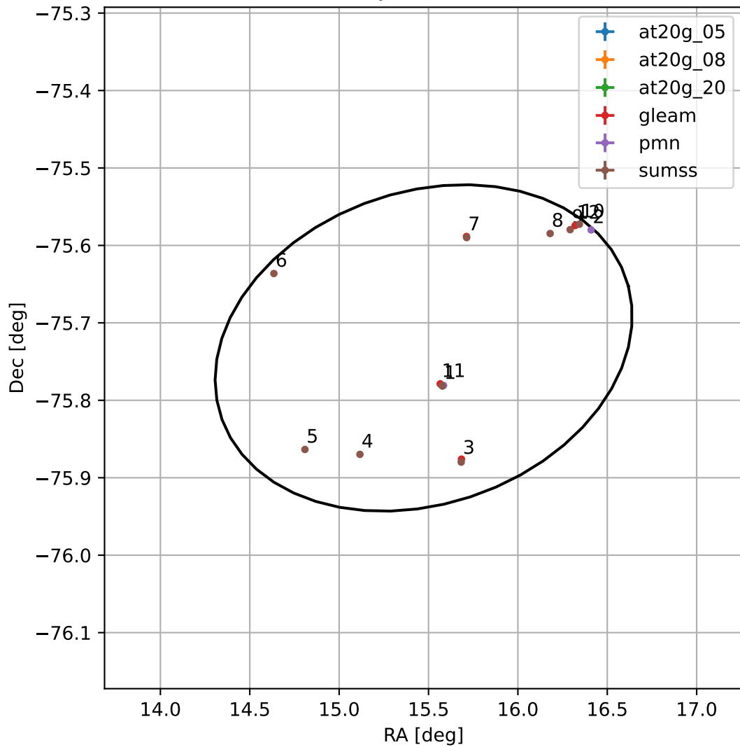
4FGL J0101.8-7543
