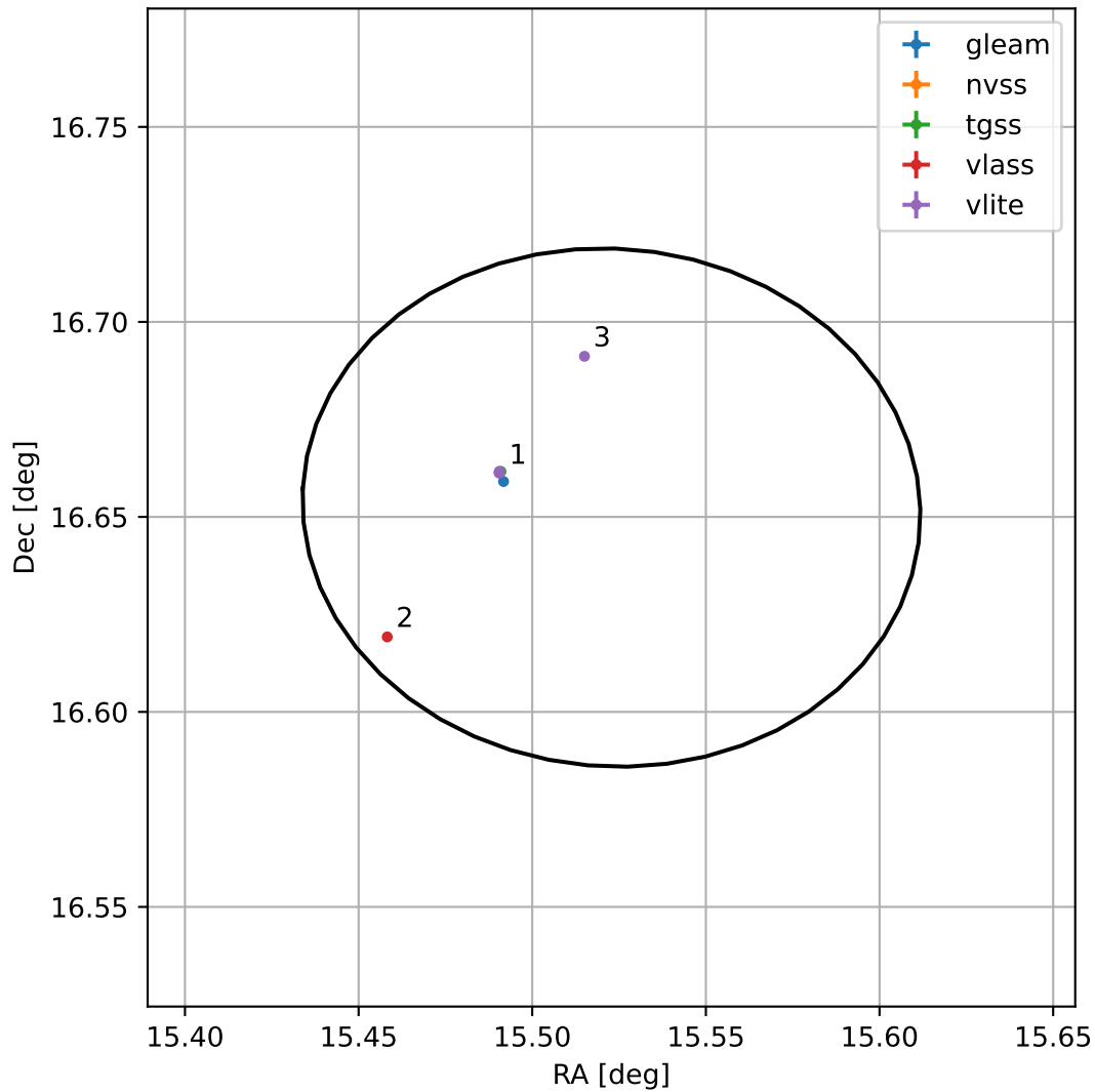
4FGL J0102.0+1639
