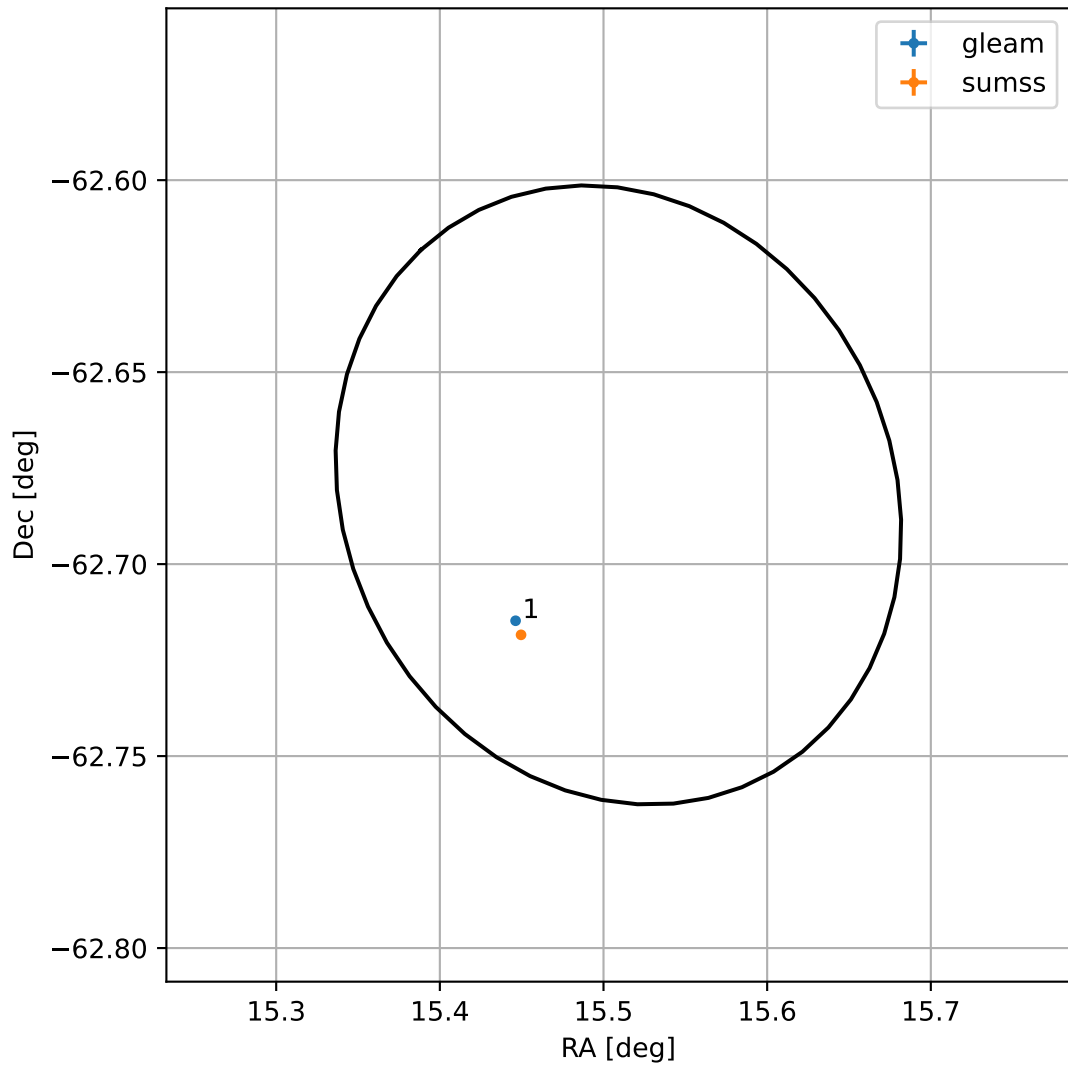
4FGL J0102.0-6240
