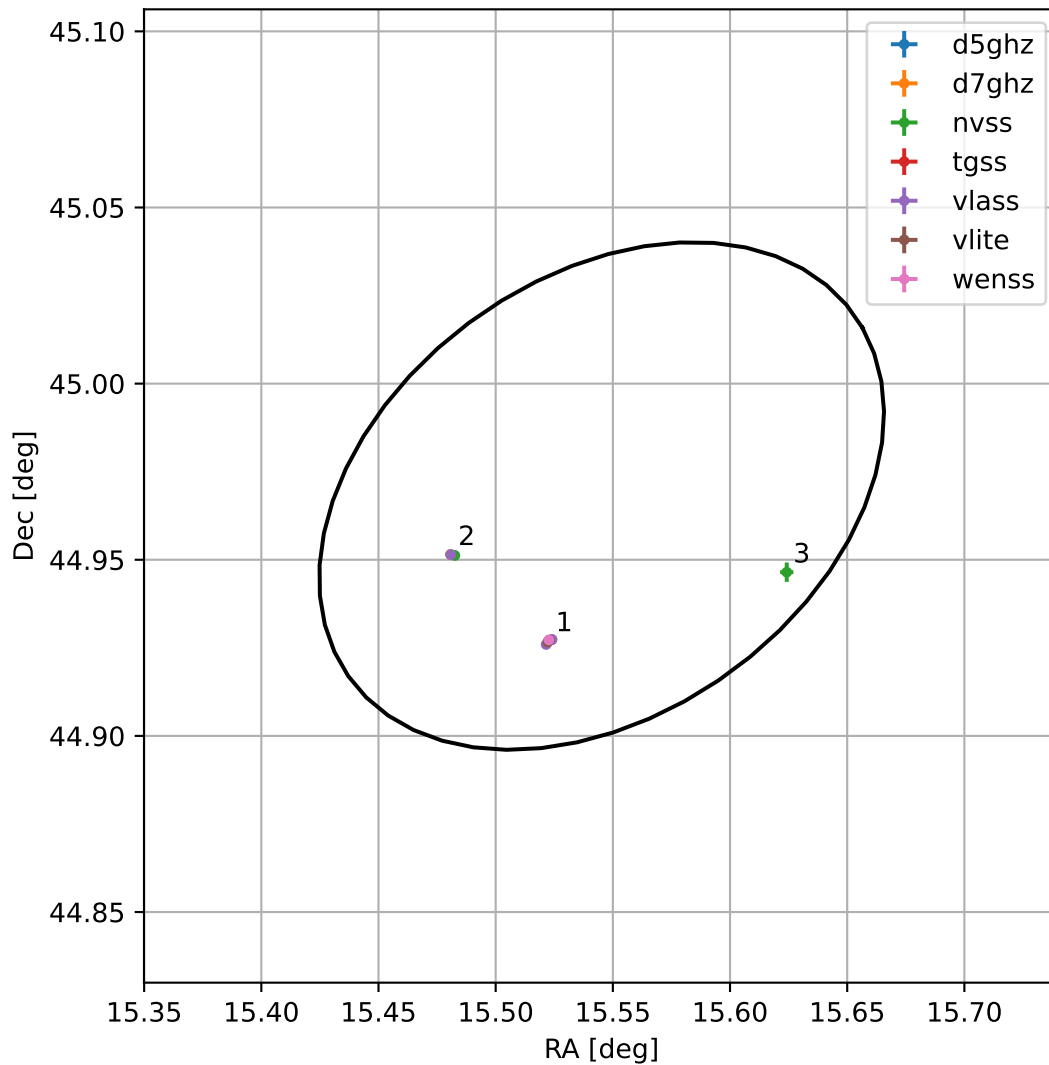
4FGL J0102.1+4458
