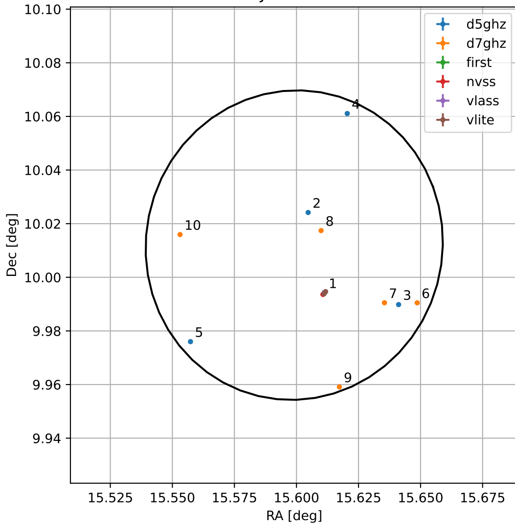
4FGL J0102.3+1000
