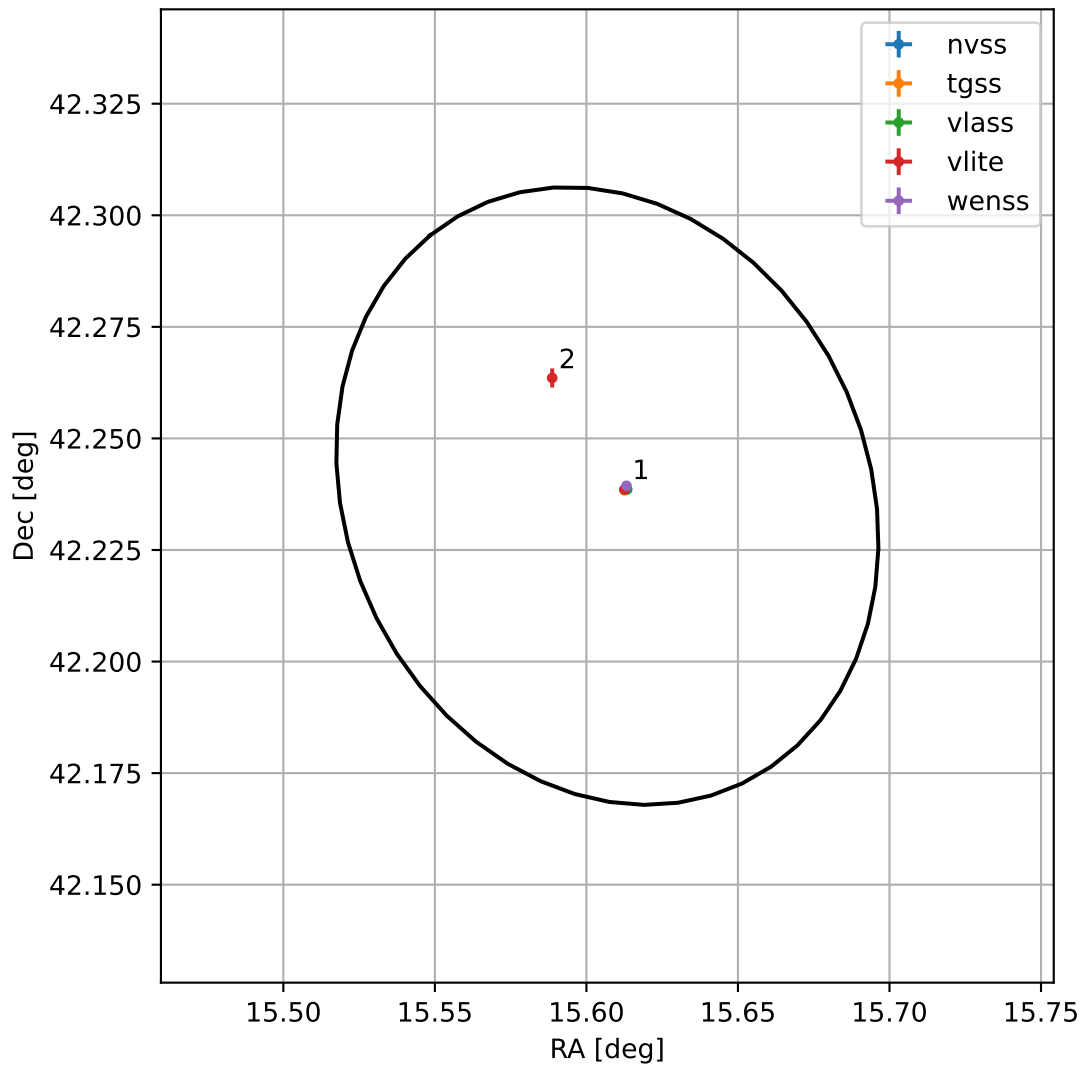
4FGL J0102.4+4214
