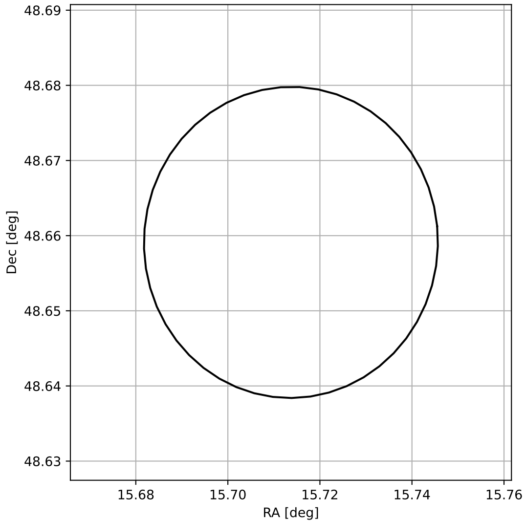
4FGL J0102.8+4839
