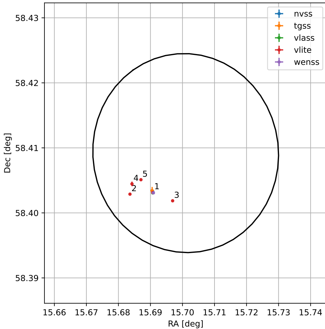
4FGL J0102.8+5824
