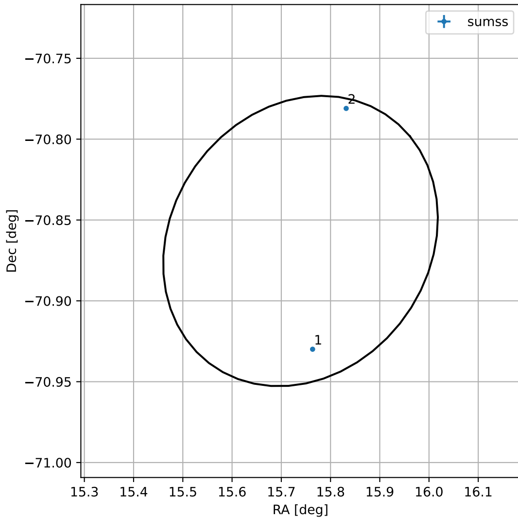
4FGL J0102.9-7051
