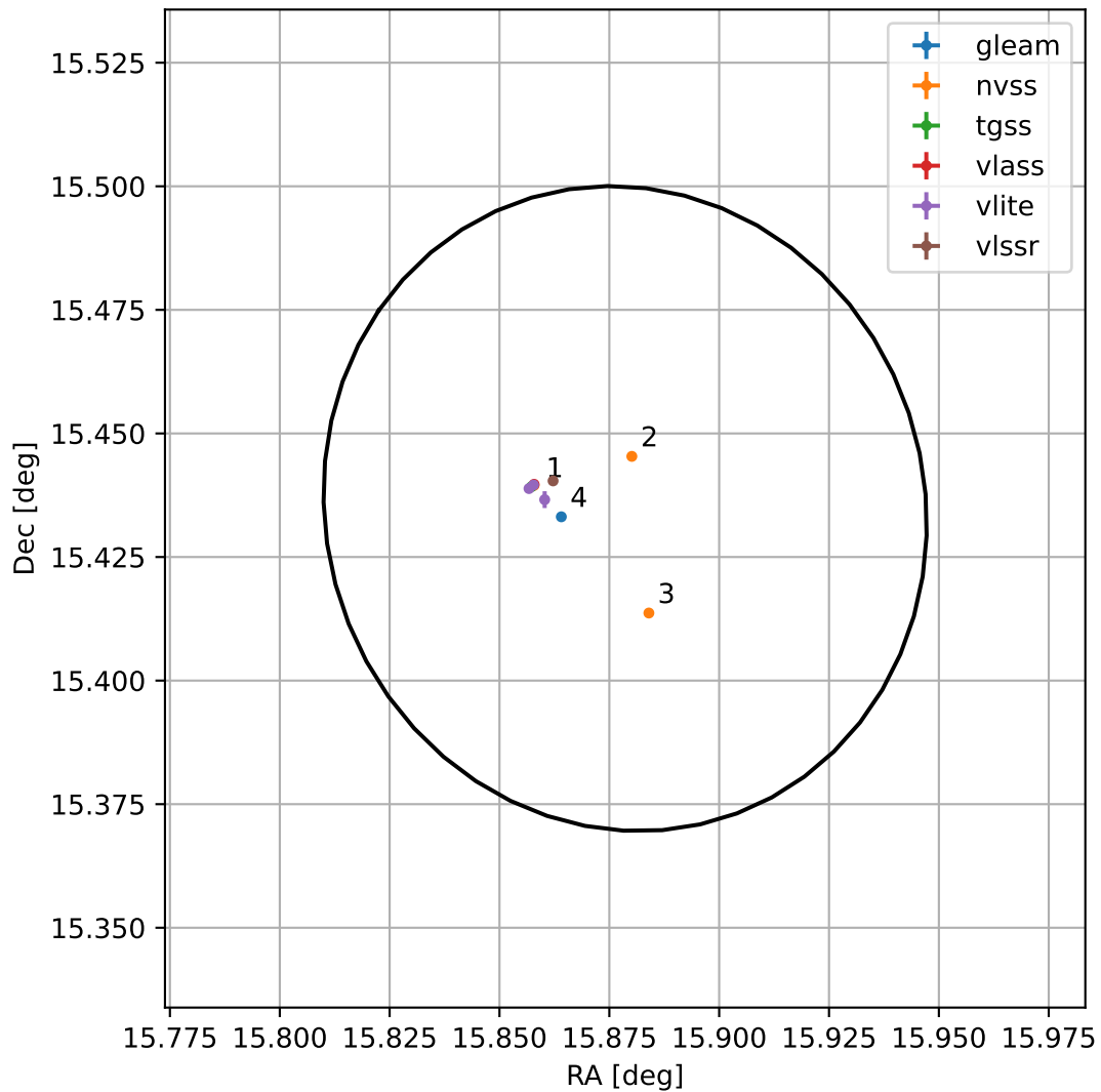
4FGL J0103.5+1526
