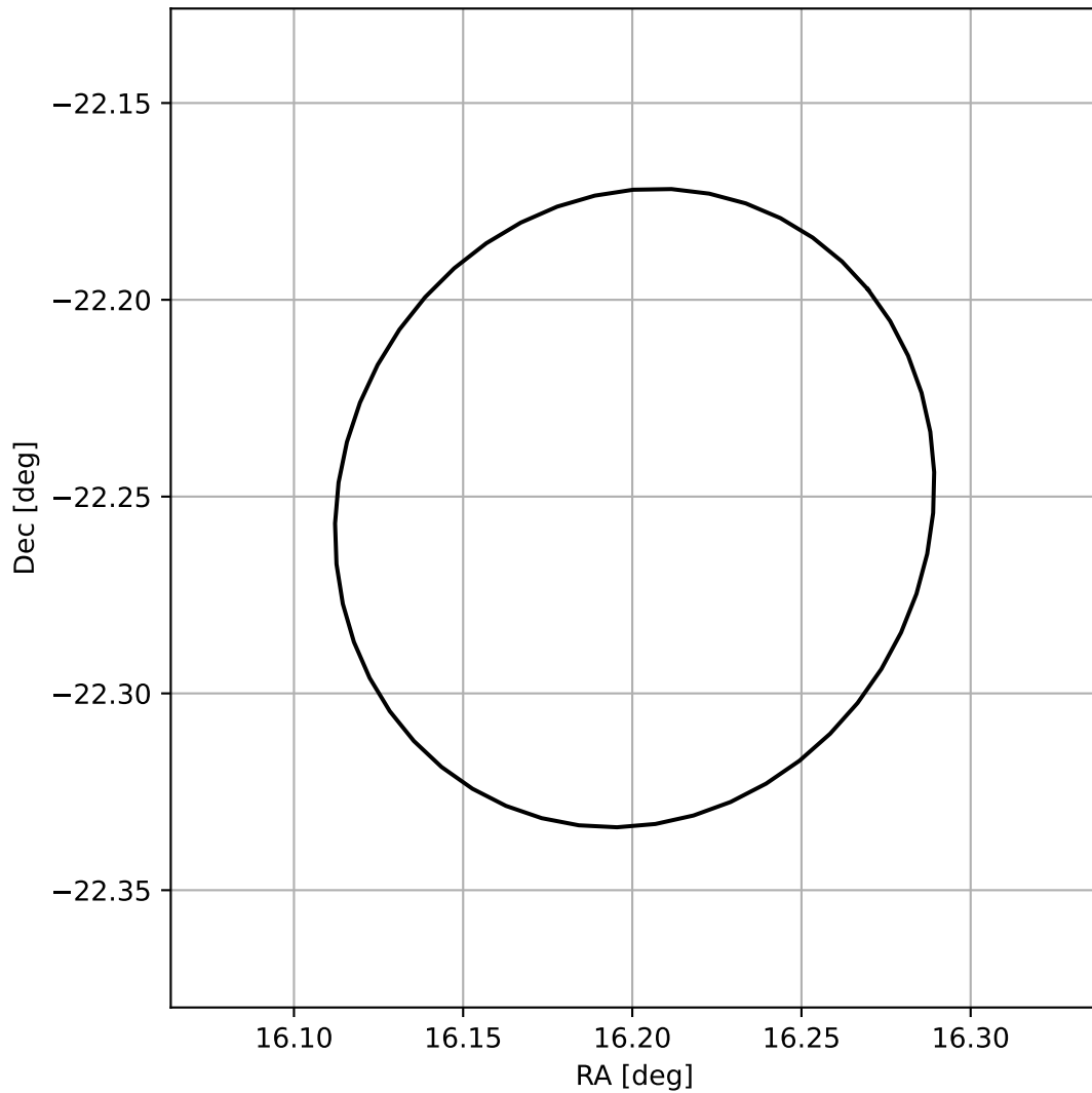
4FGL J0104.8-2215
