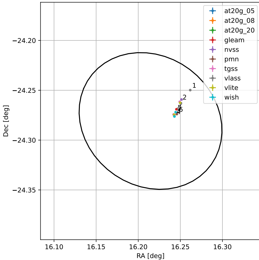
4FGL J0104.8-2416
