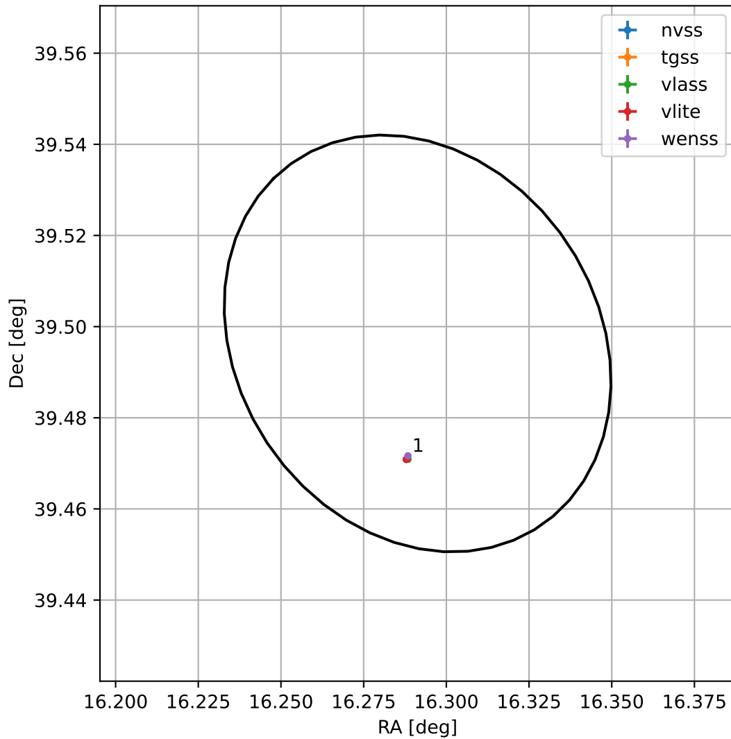
4FGL J0105.1+3929
