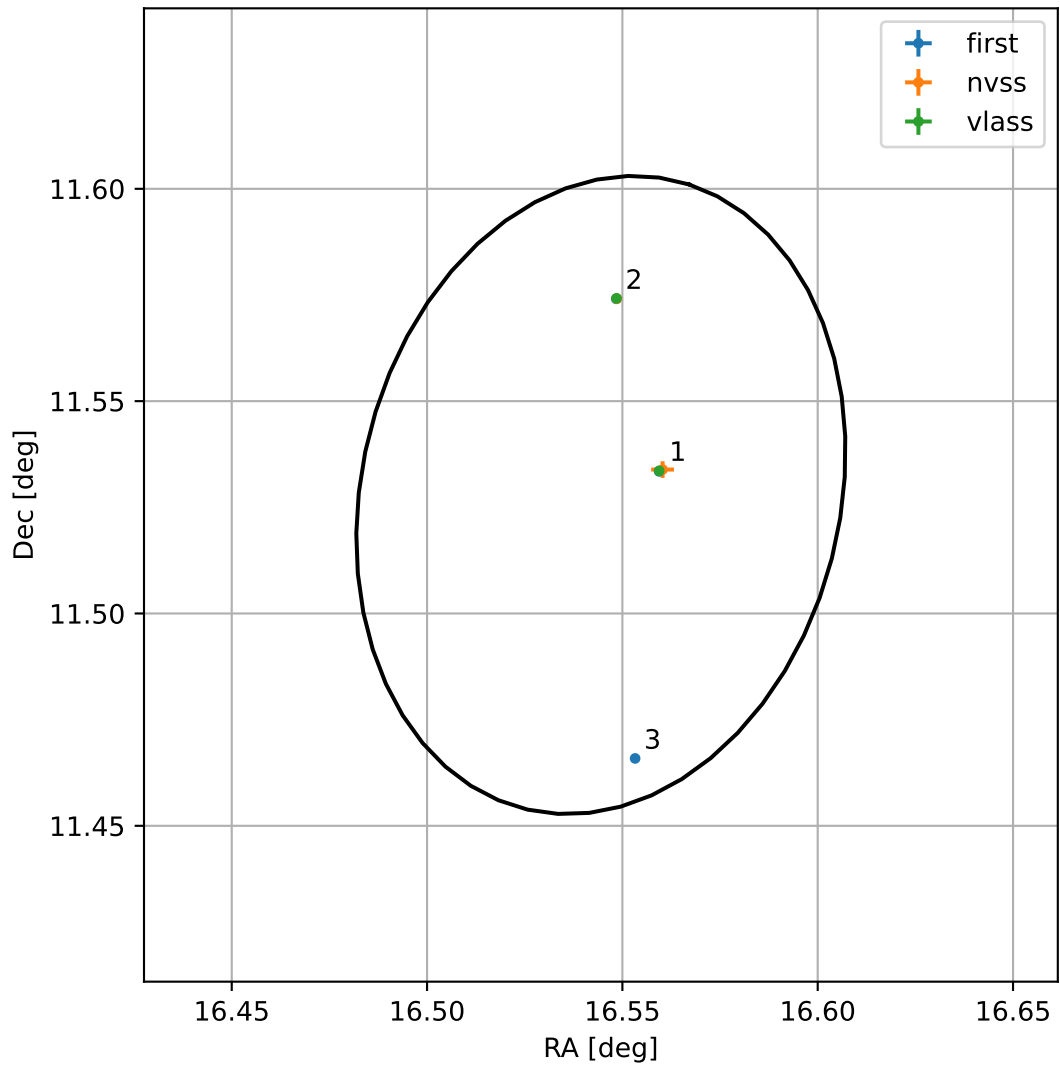
4FGL J0106.1+1131
