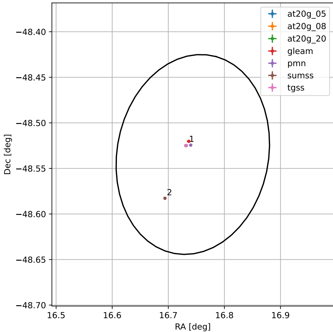
4FGL J0106.9-4832
