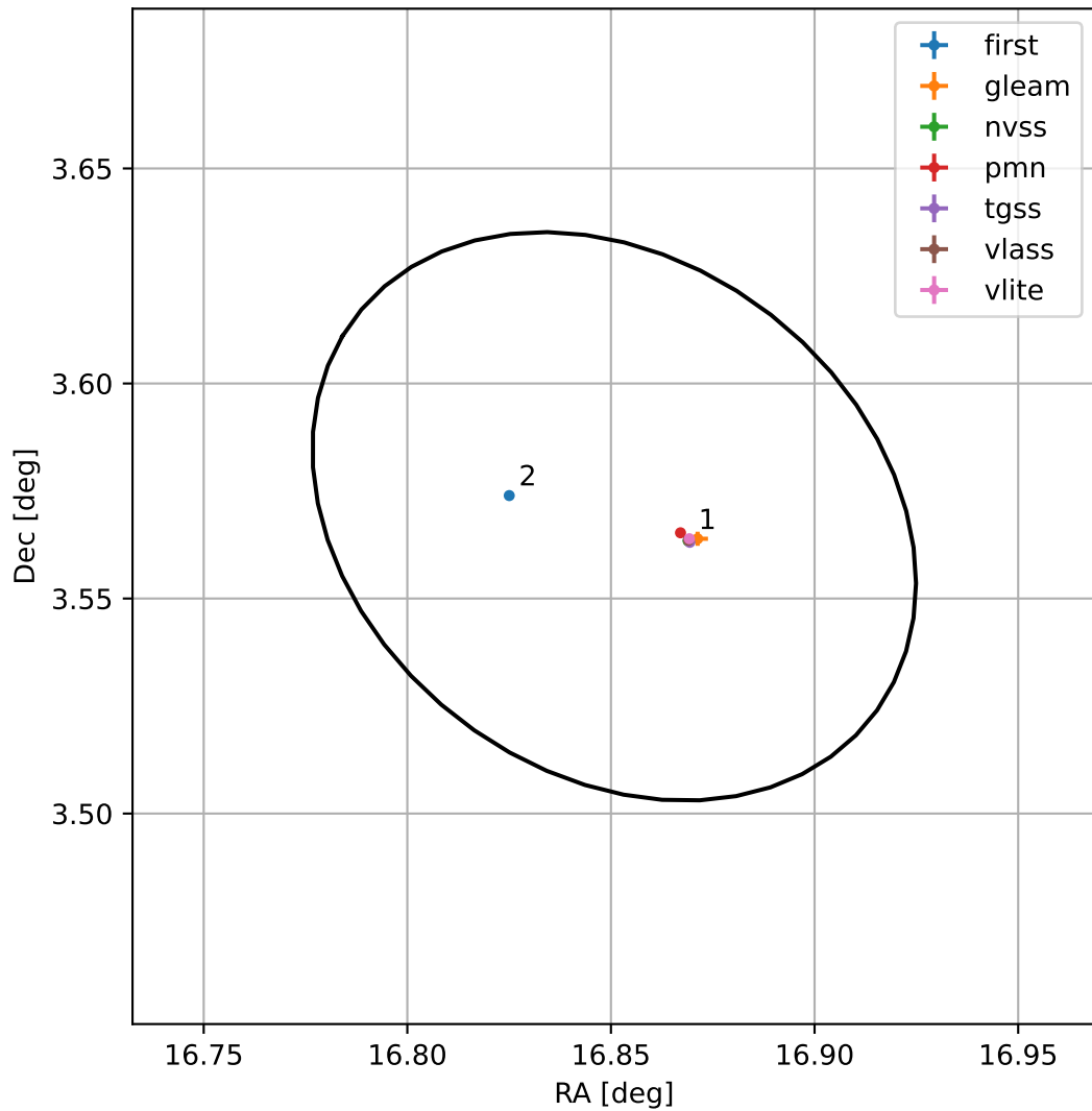
4FGL J0107.4+0334
