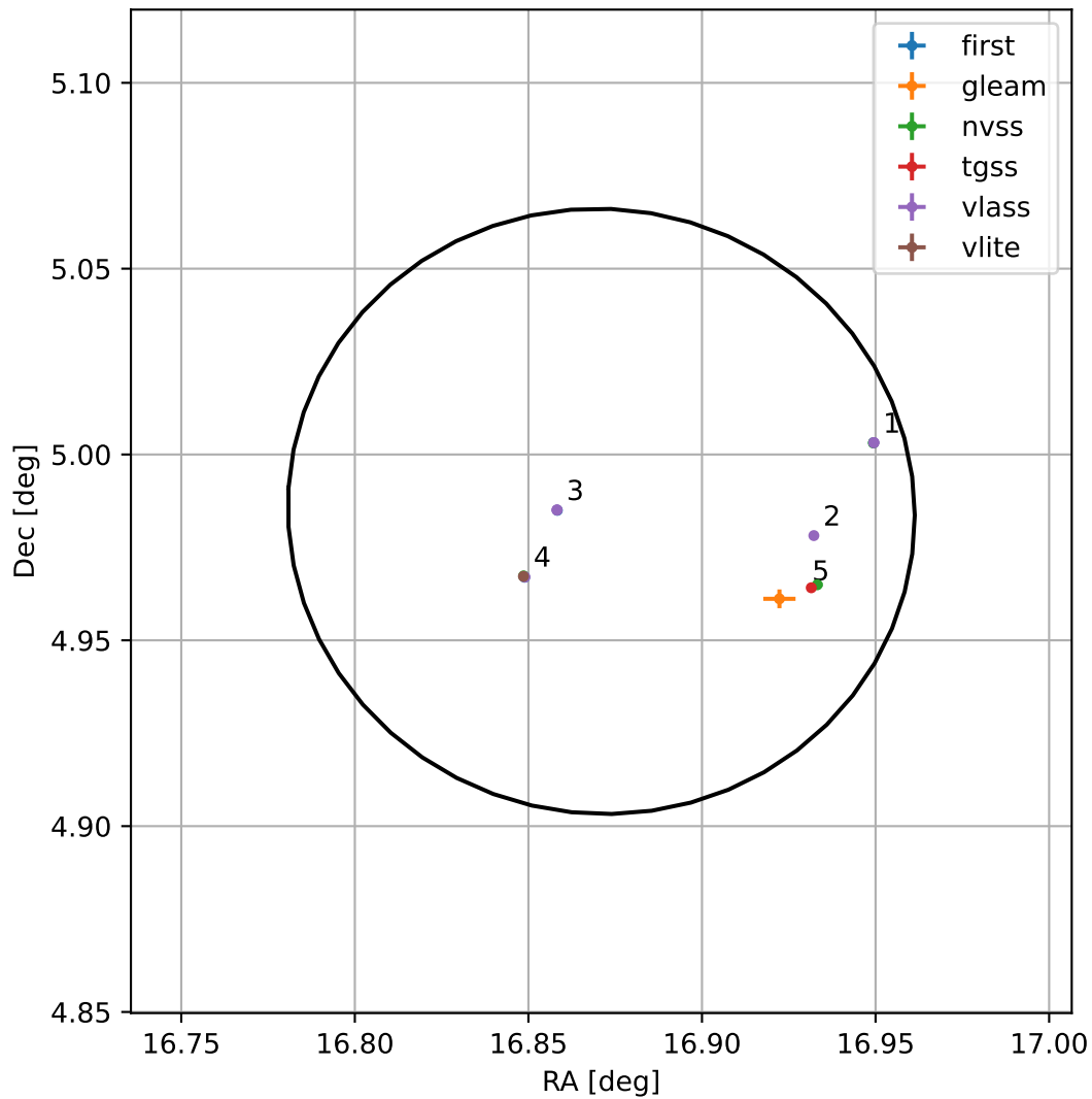
4FGL J0107.4+0459
