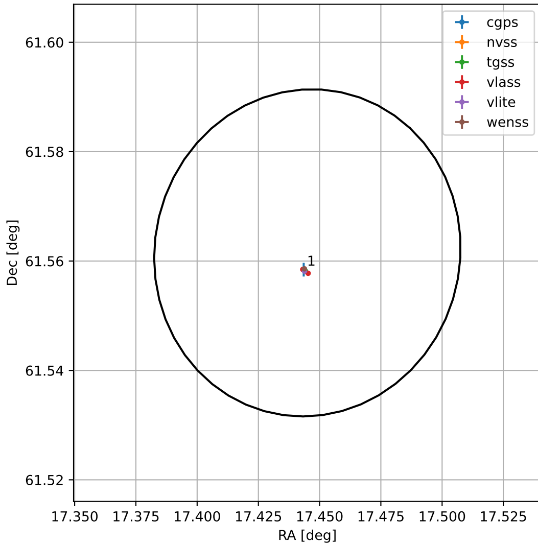
4FGL J0109.7+6133
