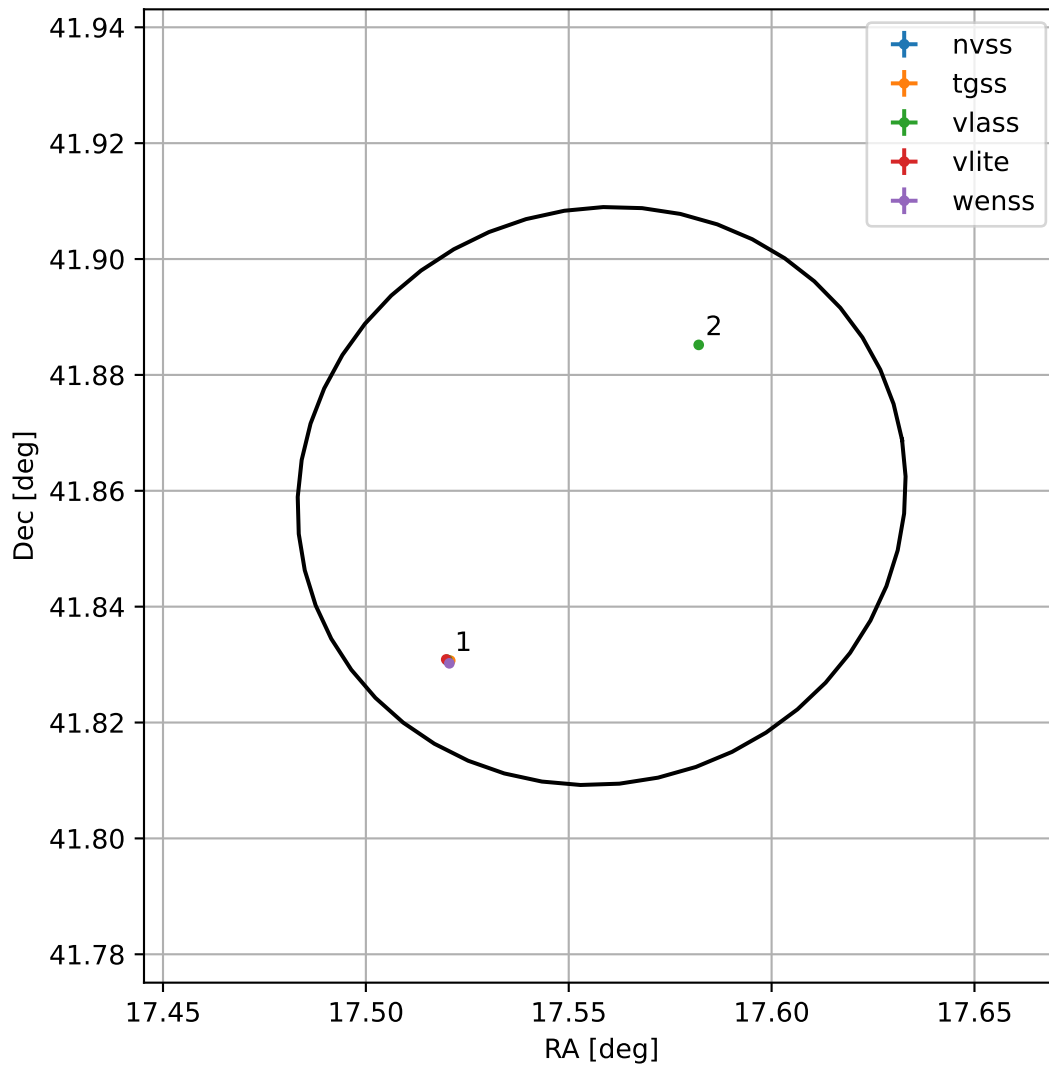
4FGL J0110.2+4151
