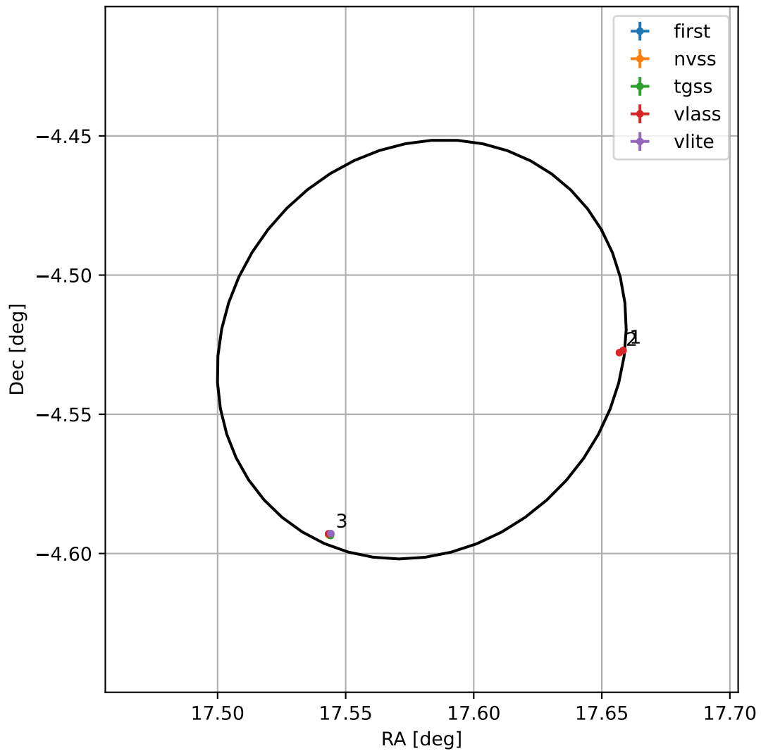
4FGL J0110.3-0431
